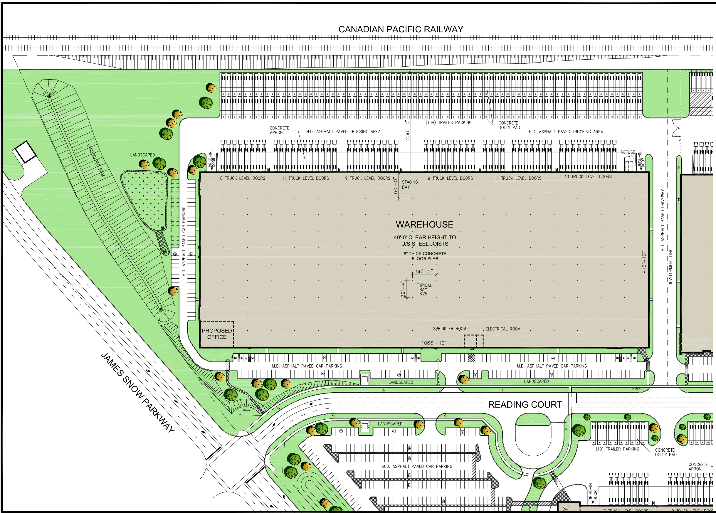
KEY PLAN
