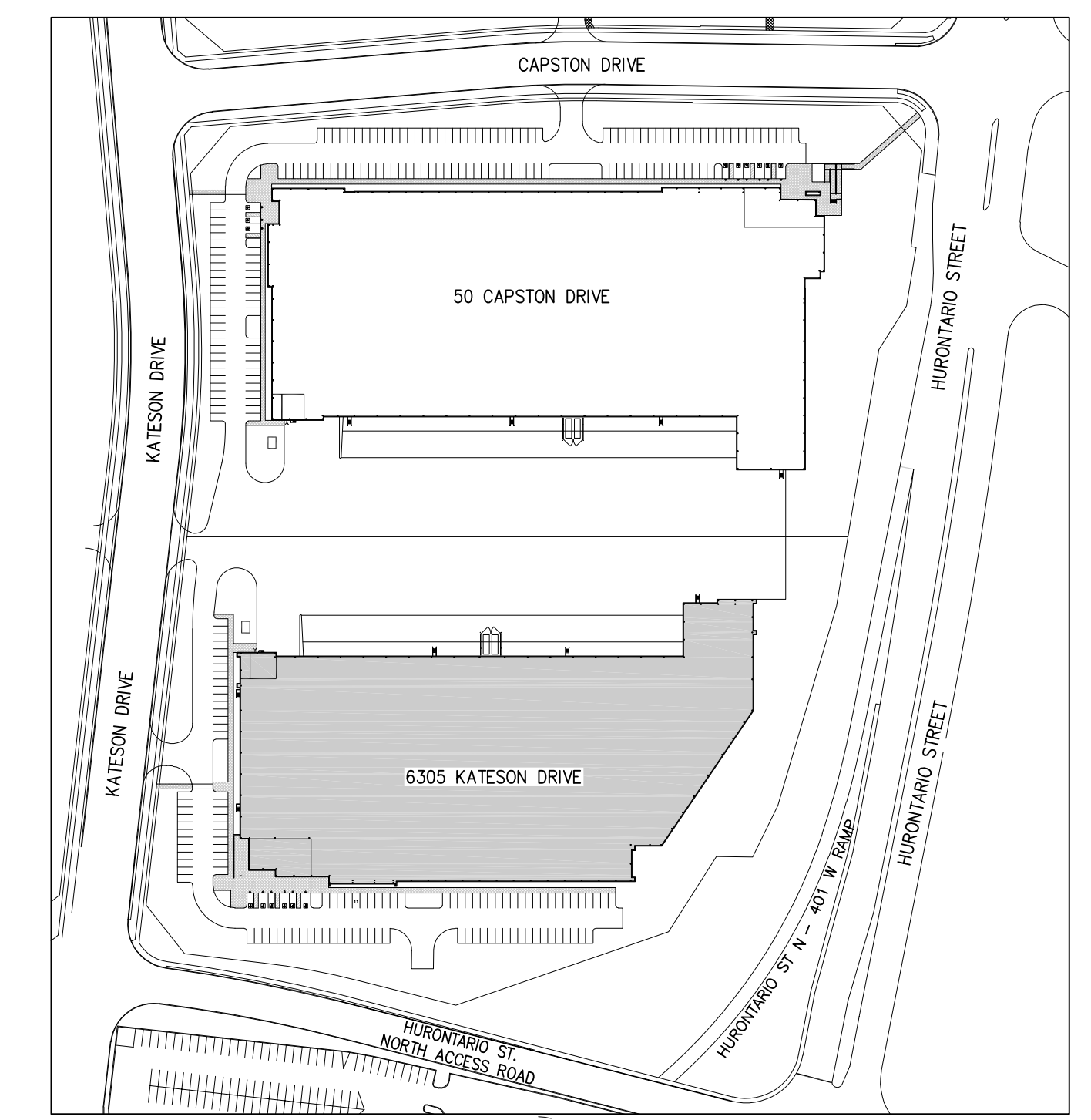
KEY PLAN
